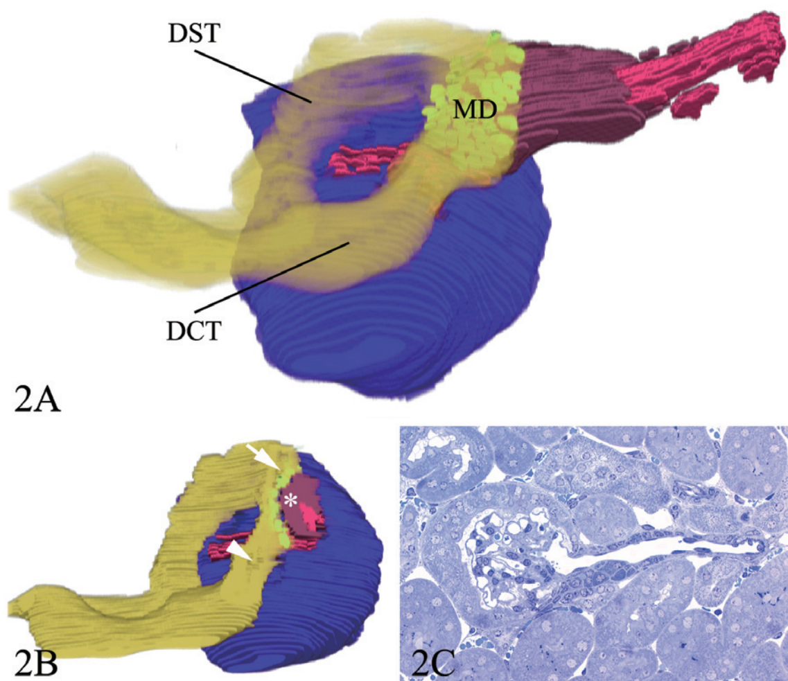
Fig. 2 Spatial arrangement of mouse juxtaglomerular ( JG ) complex and renal corpuscle reconstructed from serial epon sections. DCT: distal convoluted tubule, DST: distal straight tubule, MD: macula densa. In A, JG cells ( brown ) surround an afferent vessel ( red ) and contact with the MD ( green yellow: nuclei of MD cells ) at the vascular pole. On a cutting view( B ) , the MD is flat and exists along the JG cells. The layer of the JG cells is thick at the side of the MD ( asterisk ) This layer has been verified as two or three-cells thick by observing the serial sections used for the 3D reconstruction( C ) In B, it is interesting that the distal tubule( yellow ) becomes flat and narrow toward the MD ( arrow ) and then broad after the MD ( arrowhead ) .
